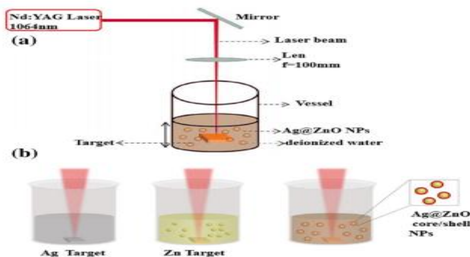
Fig. 1. (a) Schematic diagram of the PLAL setup. (b) Synthesis process of the ZnO:Ag nanostructures[49].
