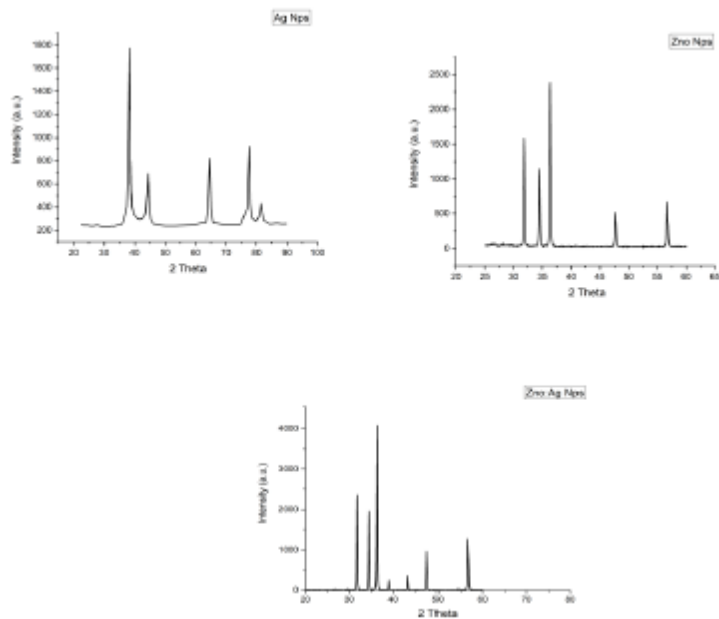
Fig 2. XRD Patterns of Ag NPs, ZnO NPs and ZnO:Ag NPs .
