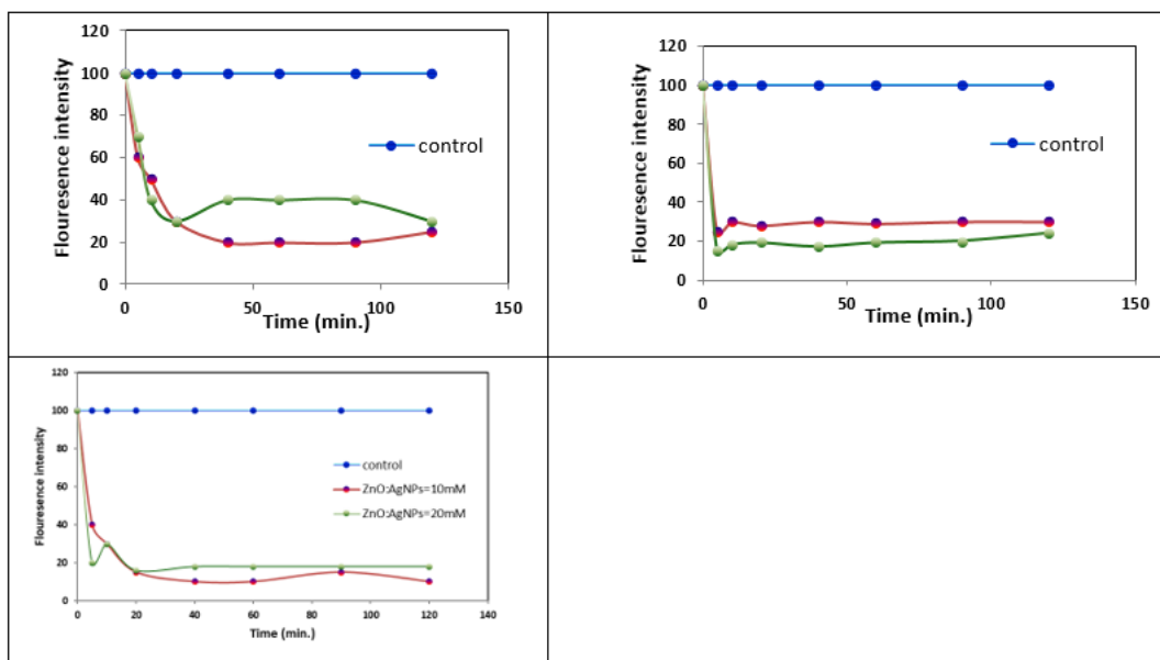
Fig. 8. fluorescence intensity rate as a function of incubation time and concentration of ZnO NPs and ZnO:Ag
