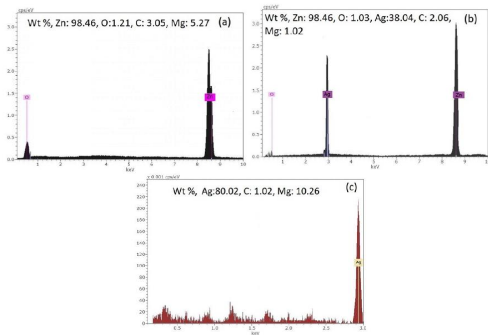
Fig. 7. EDX Spectrum of (A) ZnO, (B) Ag NPs and (C) ZnO: Ag NPs.
